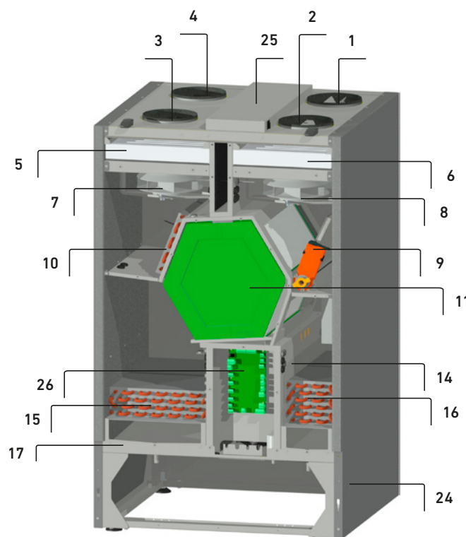
PKOM 4 TREND (RIGHT-HANDED VERSION)
