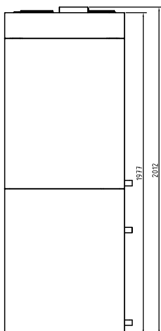
Illustration: PKOM 4 classic (right-handed design)
