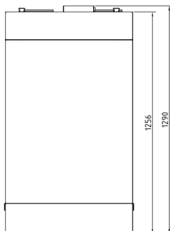
Illustration: PKOM 4 trend (right-handed design)
