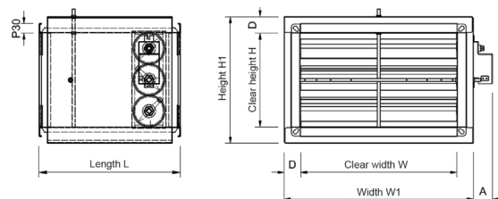
PVSR-EJ/D - with insulating shell
