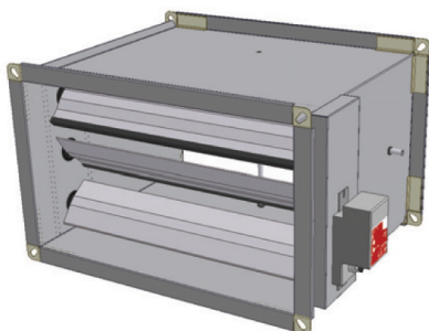
PVSR-EJ - without insulating shell
