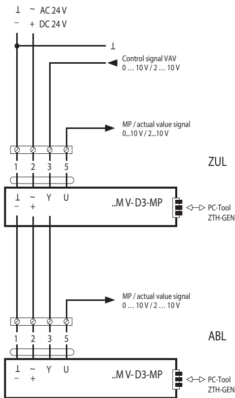
Example 3: VAV with analogue control signal ZUL/ABL connected in parallel
