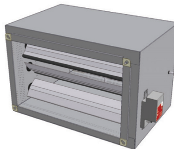
PVSR-EJ/D - with insulating shell
