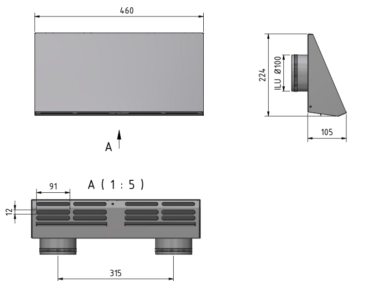
When using the ODA/EHA connecting piece DN100
