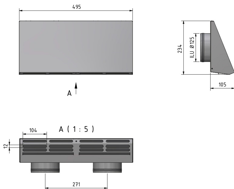
When using the EPP wall duct element
