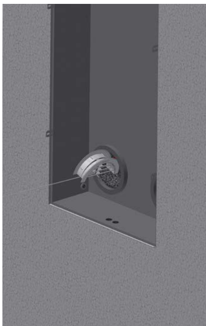
Leading the plastic grille NW170 through the aperture
