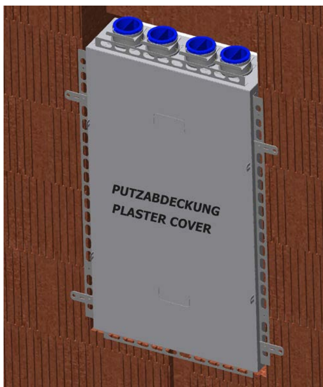
Mounted dirt cover
