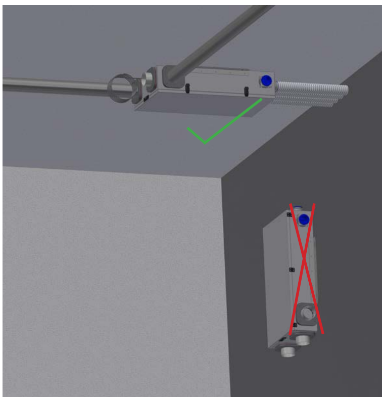
Observe the position of the unit
