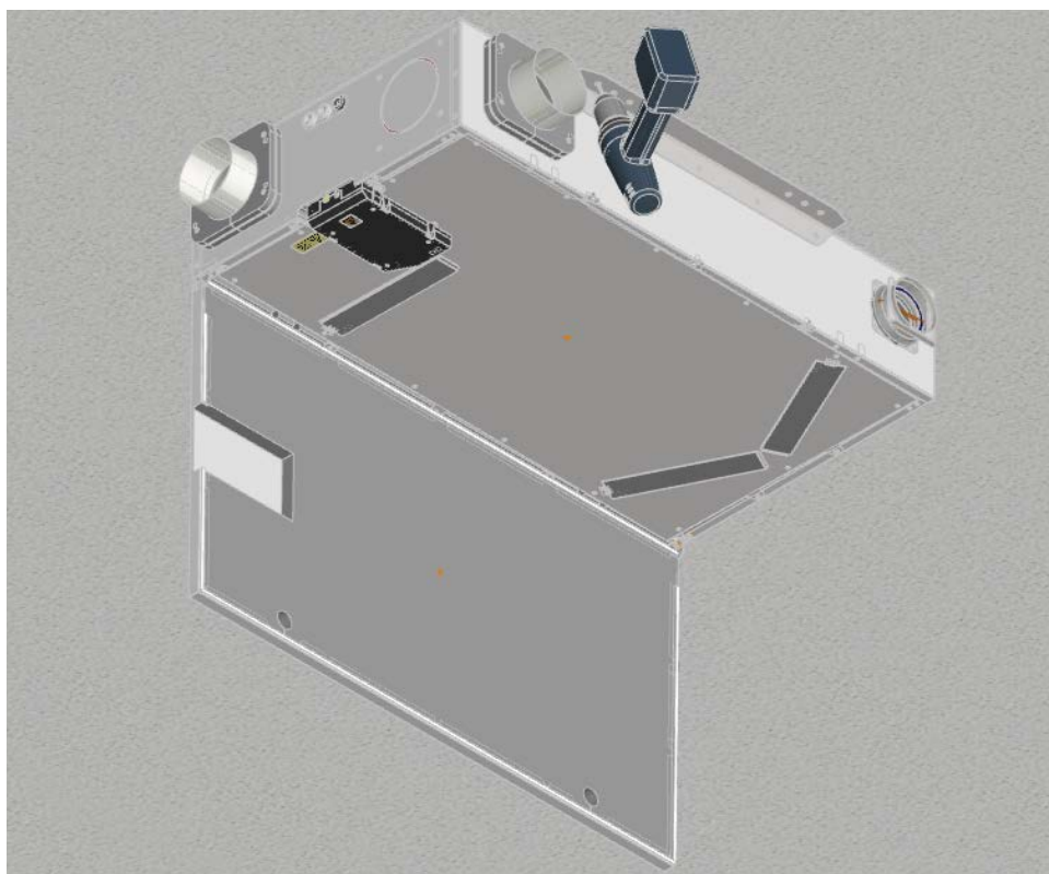
Installation of the unit on the ceiling
