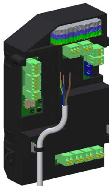
Fix the mains supply line using cable ties
