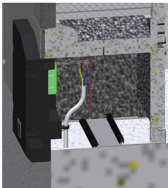
Disassemble the control housing
