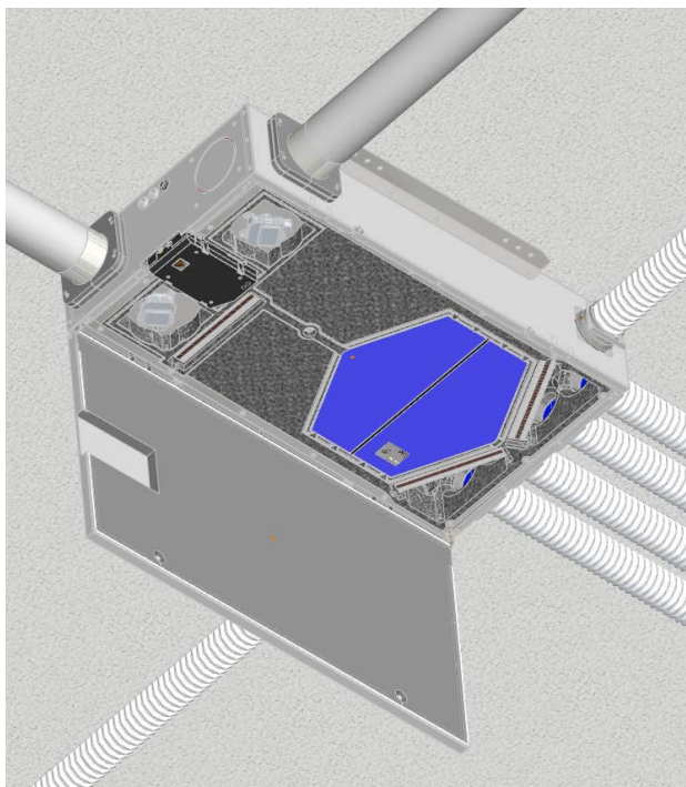
Ceiling unit without sealing plate
