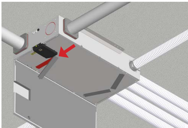
Remove the filter cover
