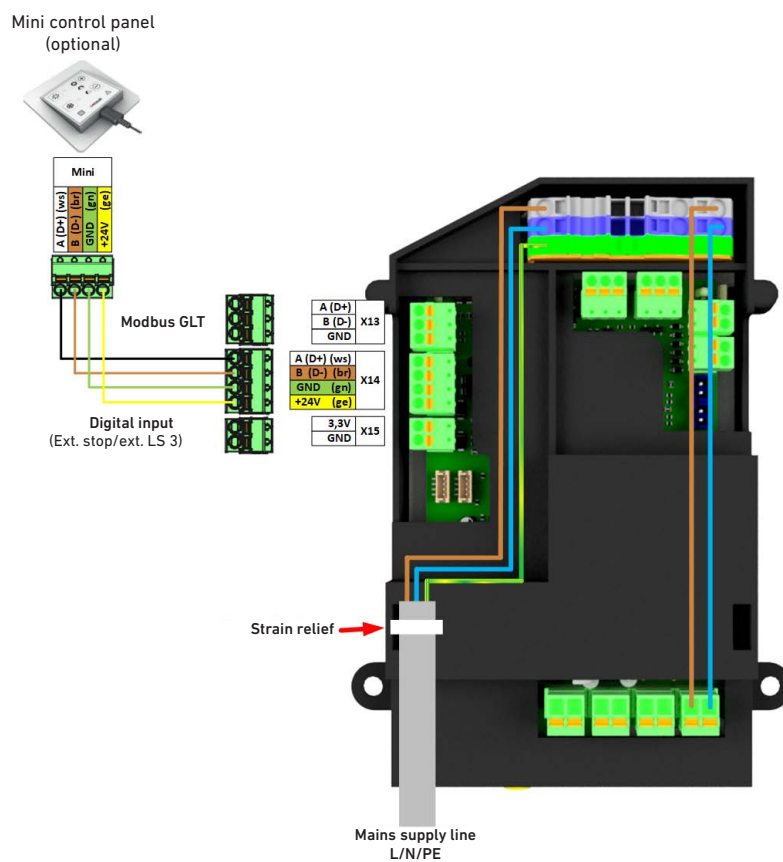
Connection diagram
