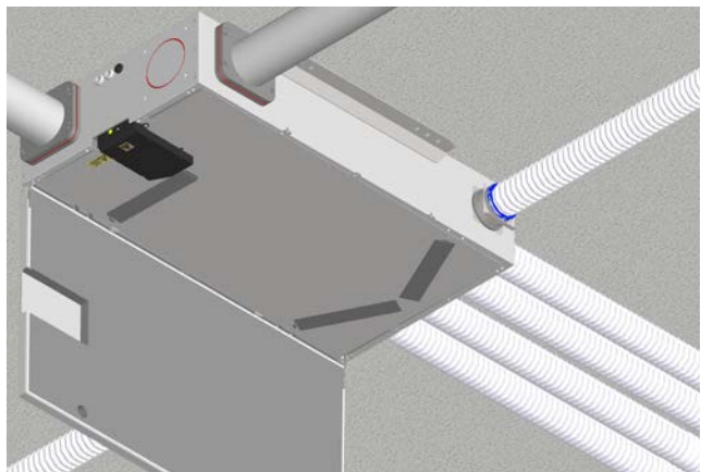
Open the swivelling cover
